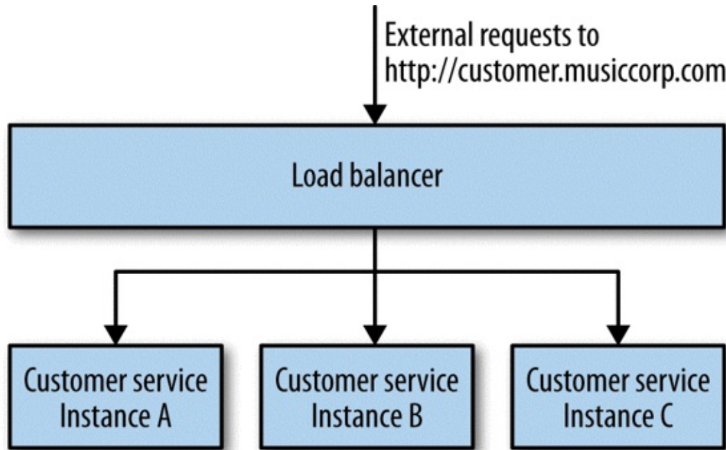
Figure 11-4. An example of a load balancing approach to scale the number of customer service instances
