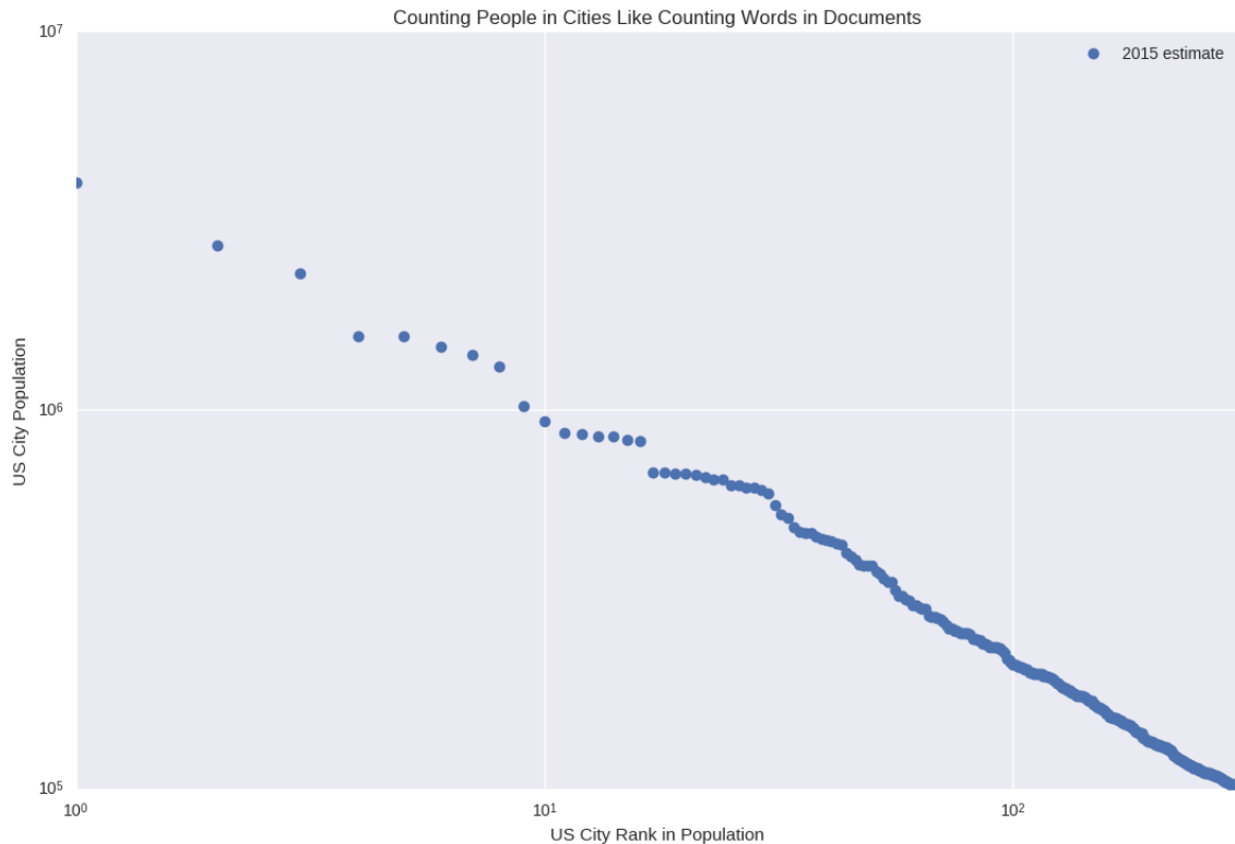
Figure 3.4 City population distribution
