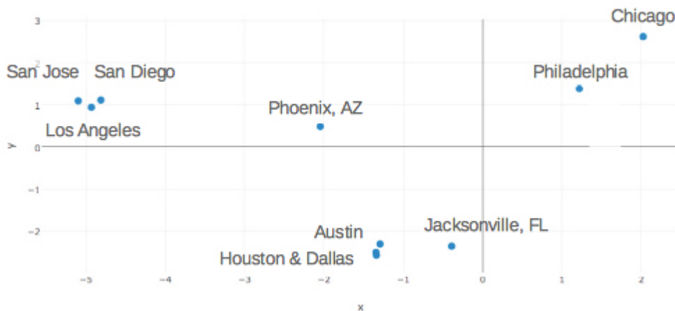
Figure 6.3 Word vectors for ten US cities projected onto a 2D map
