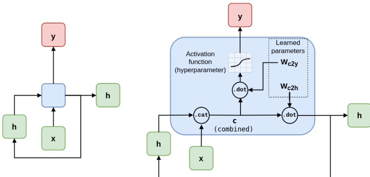
Figure 8.6 A neuron with recurrence
