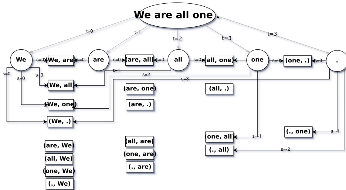
Figure 6.6 Training input and output example for the skip-gram approach
