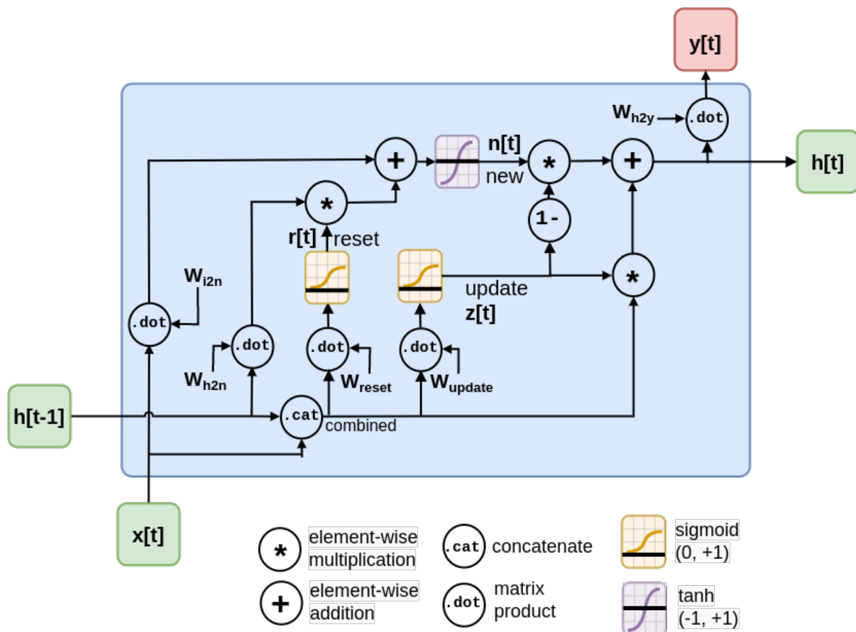
Figure 8.11 GRUs add capacity with logic gates
