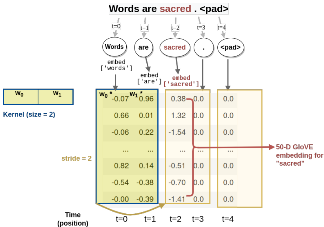
Figure 7.16 Word embeddings for convolution
