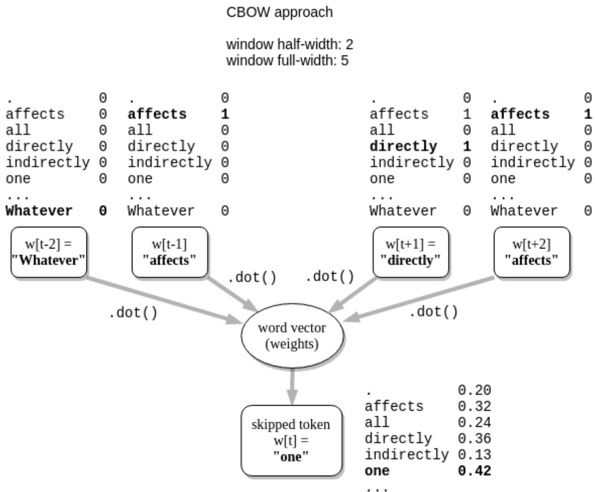
Figure 6.4 CBOW neural network architecture
