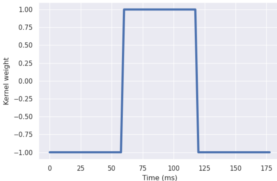
Figure 7.11 Morse code dot detecting kernel
