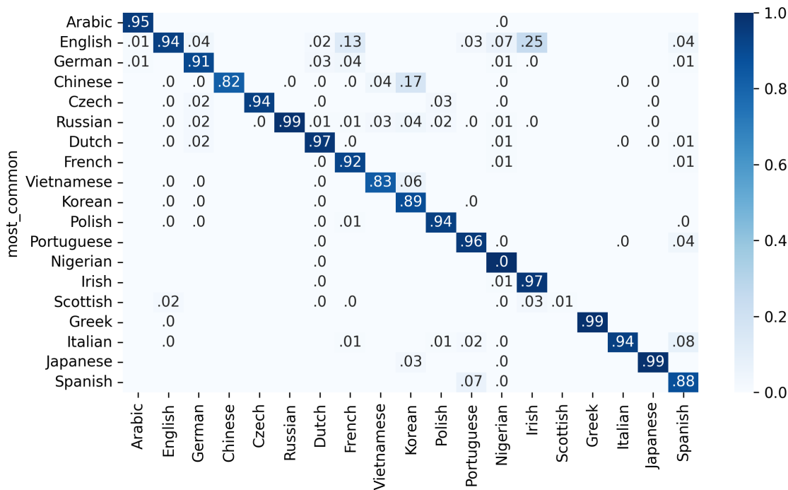
Figure 8.8 The dataset is confused even before training
