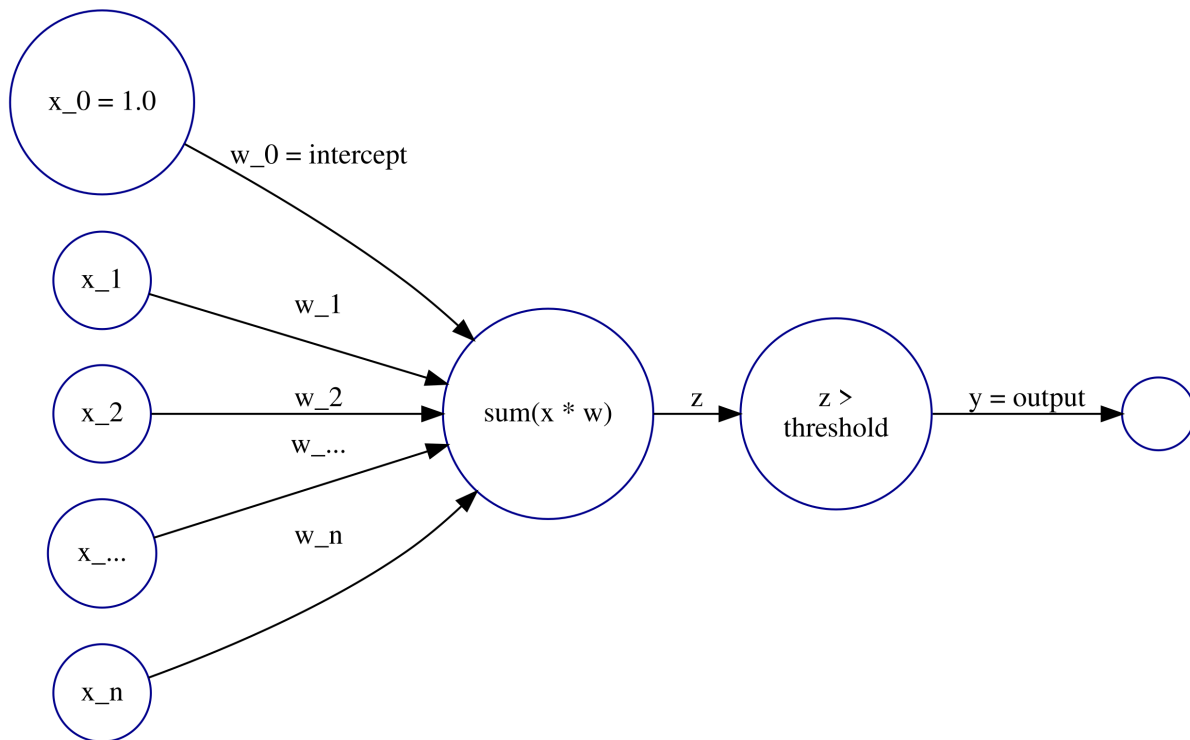
Figure 5.2 Basic perceptron
