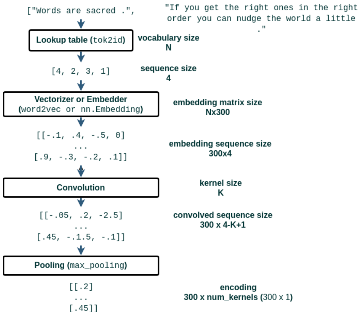
Figure 7.14 CNN processing layers 285
