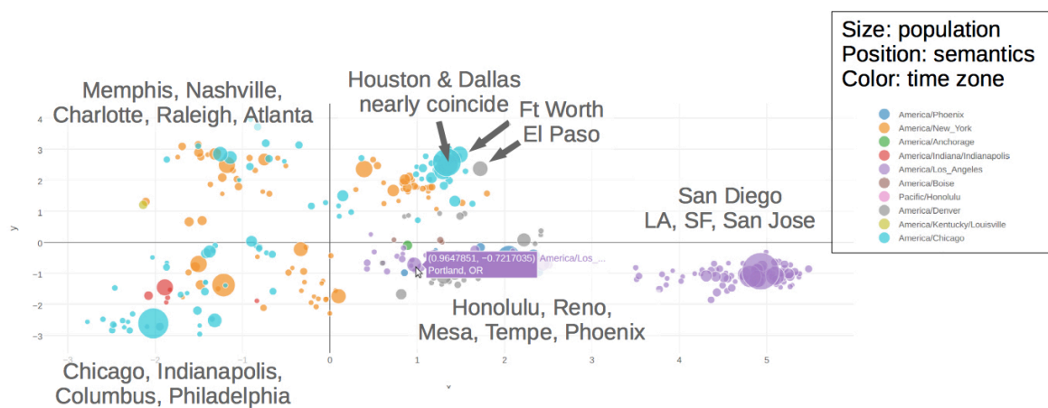
Figure 6.8 Google News Word2Vec 300-D vectors projected onto a 2D map using PCA
