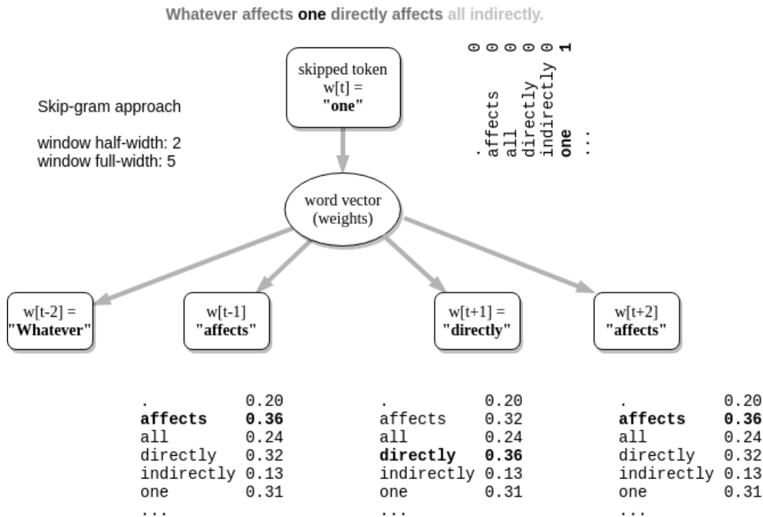
Figure 6.5 Skip-gram neural network architecture
