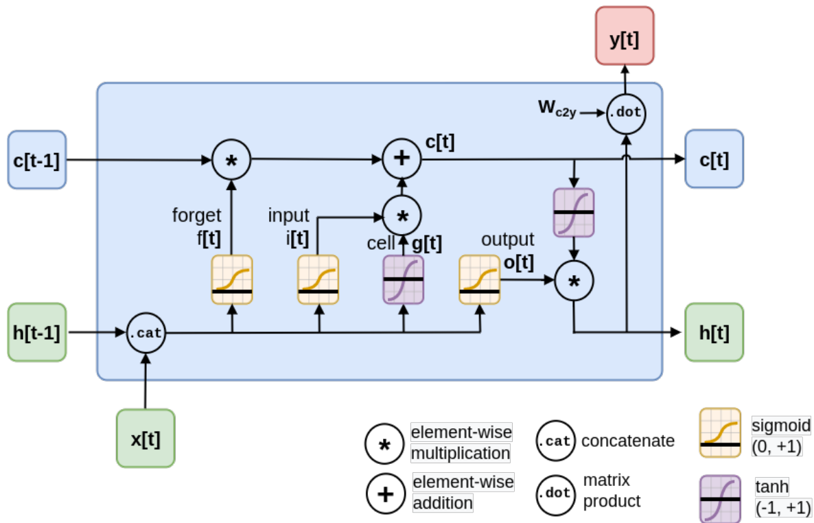
Figure 8.12 LSTMs add a forgetting gate and a cell output
