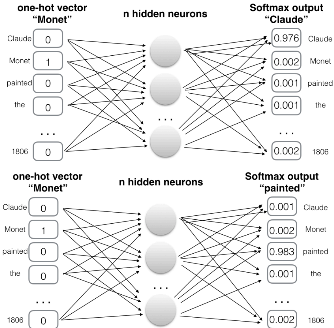
Figure 6.7 Network example for the skip-gram training
