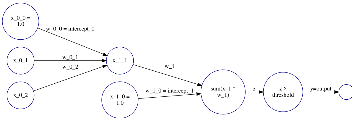
Figure 5.3 Neural network layers
