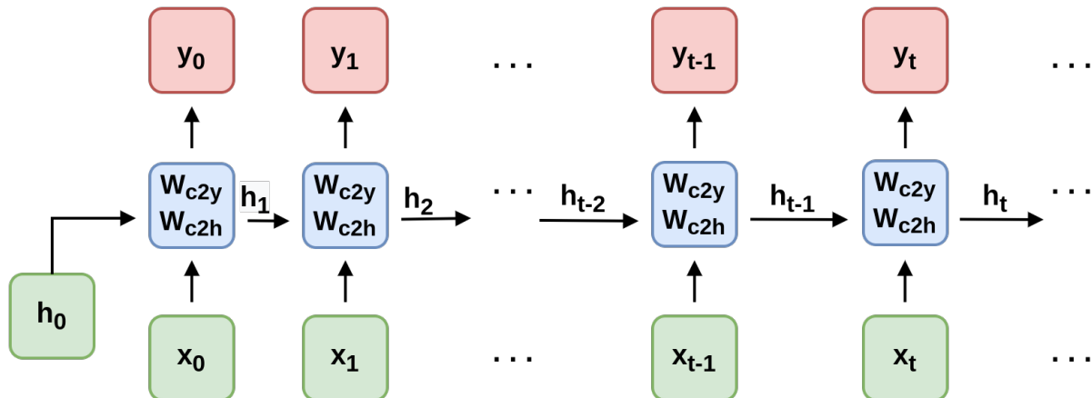
Figure 8.7 Unroll an RNN to reveal its hidden secrets
