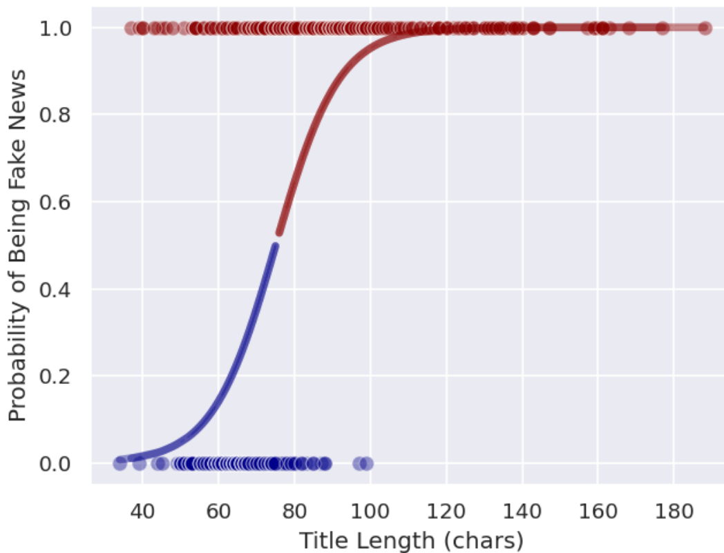
Figure 5.5 Logistic regression - fakeness vs title length
