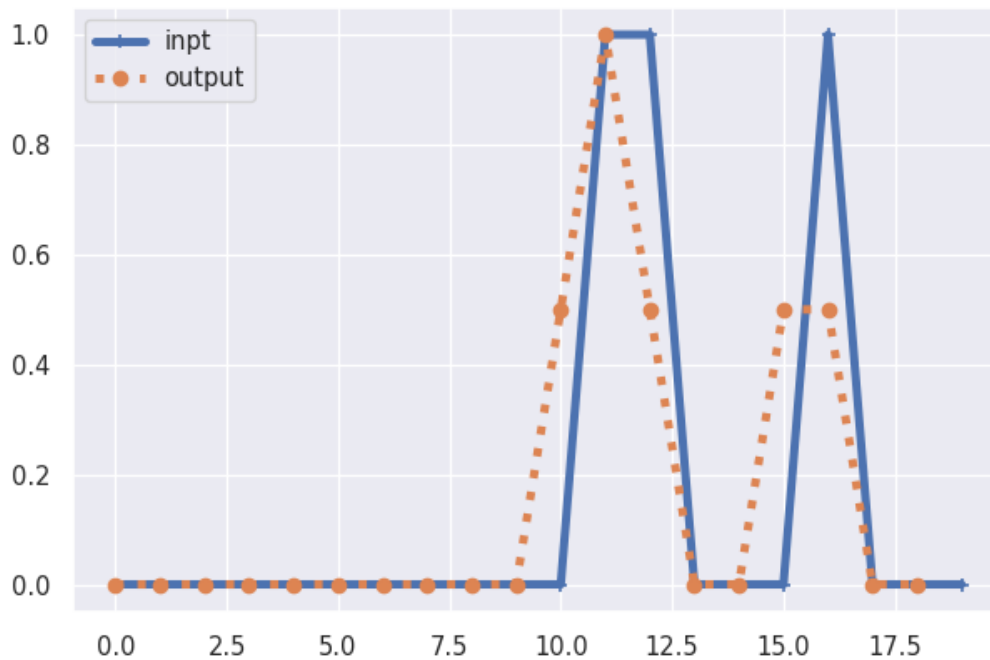
Figure 7.2 Line plot of is_adv and adverbiness convolution
