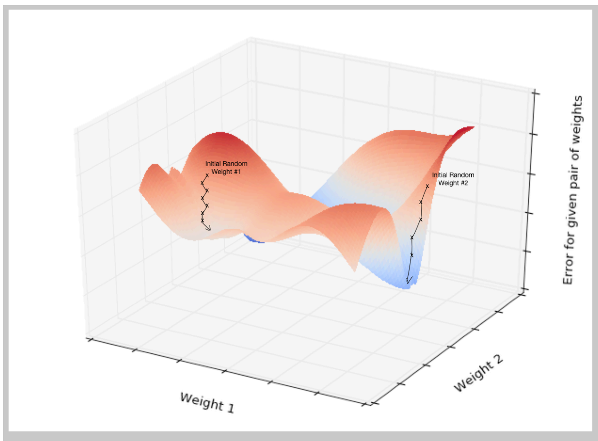
Figure 5.7 Nonconvex error curve
