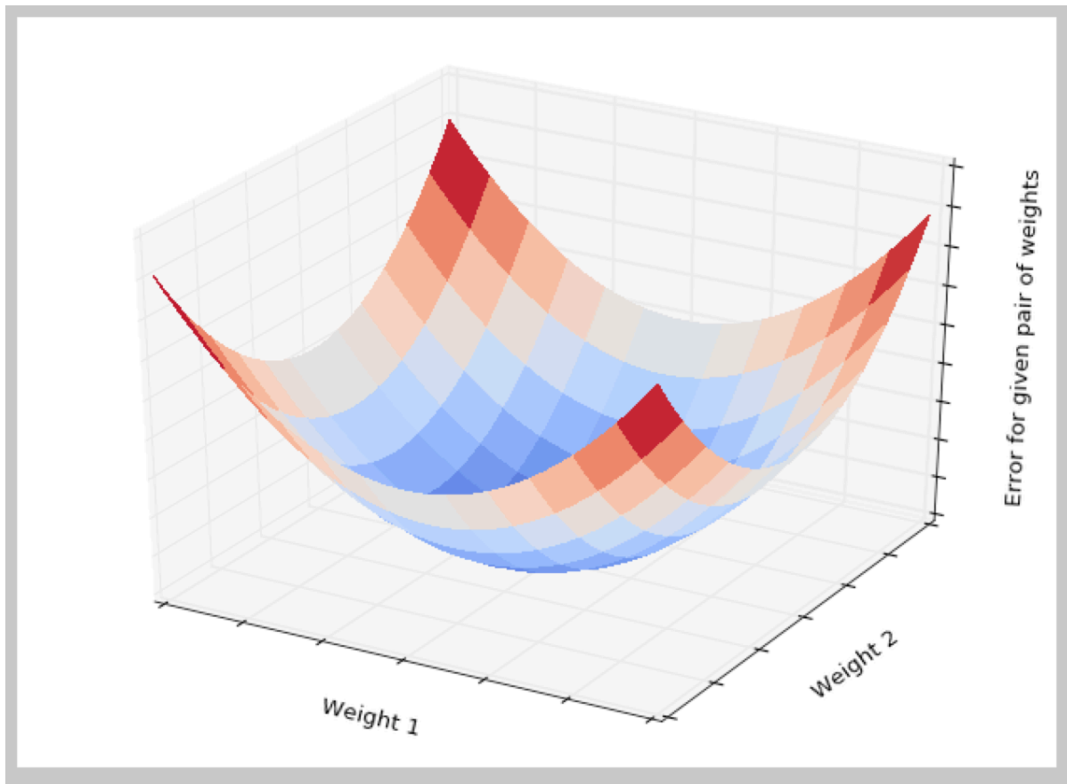
Figure 5.6 Convex error curve
