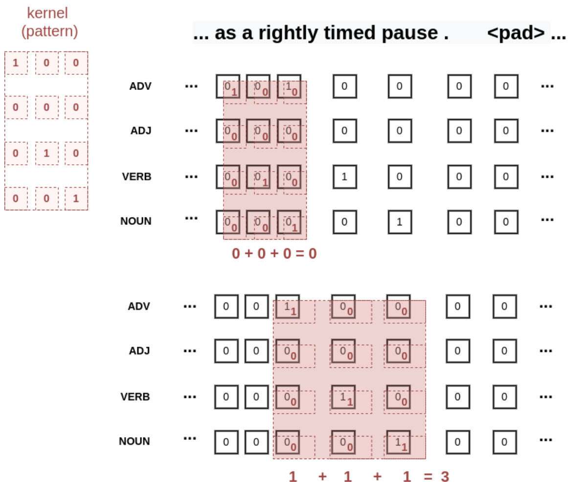
Figure 7.4 Check the convolution pattern match yourself
