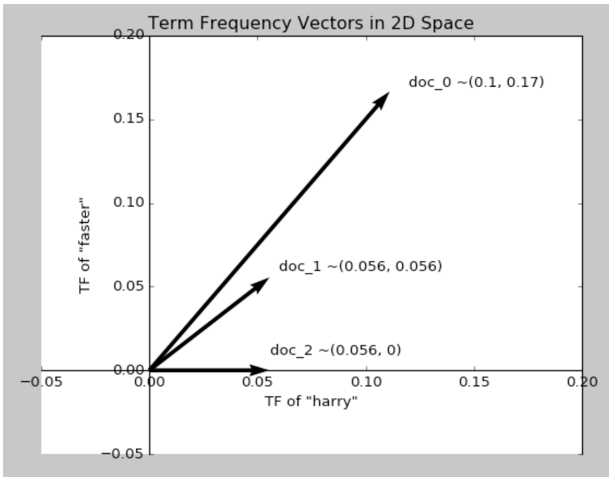
Figure 3.2 2D term frequency vectors
