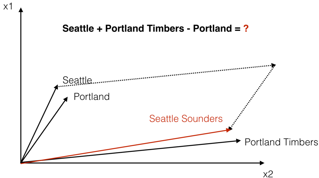
Figure 6.2 Geometry of Word2Vec math
