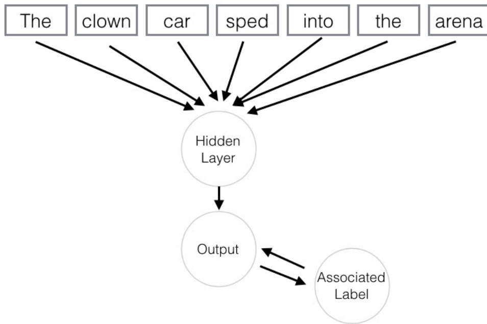
Figure 8.10 Data fed into a recurrent network
