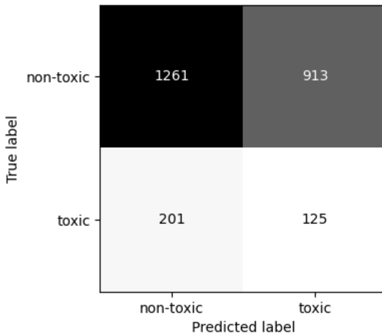
Figure 4.2 Confusion matrix of TF-IDF based classifier
