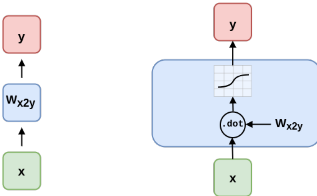
Figure 8.5 Ordinary feedforward neuron
