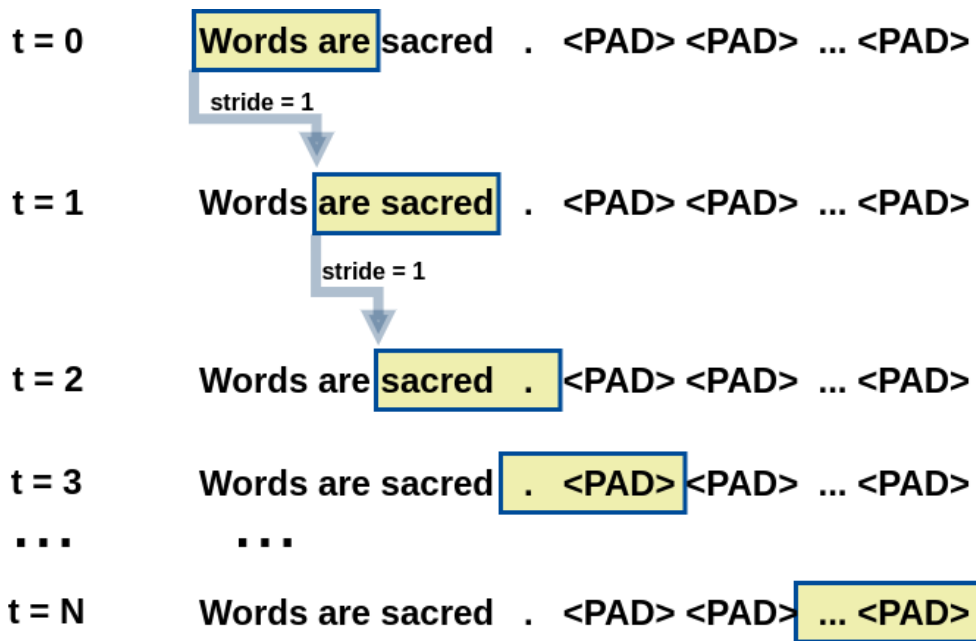
Figure 8.9 1D convolution with embeddings
