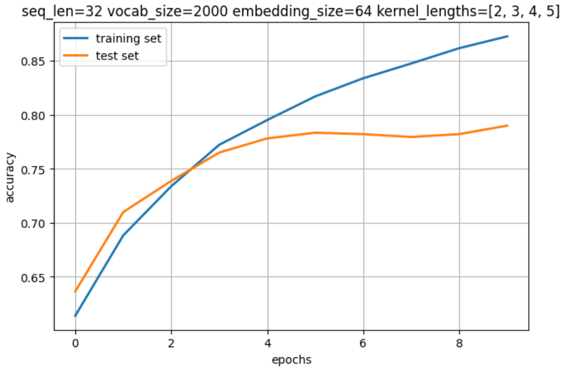
Figure 7.17 Learning curve for the best hyperparamters we found
